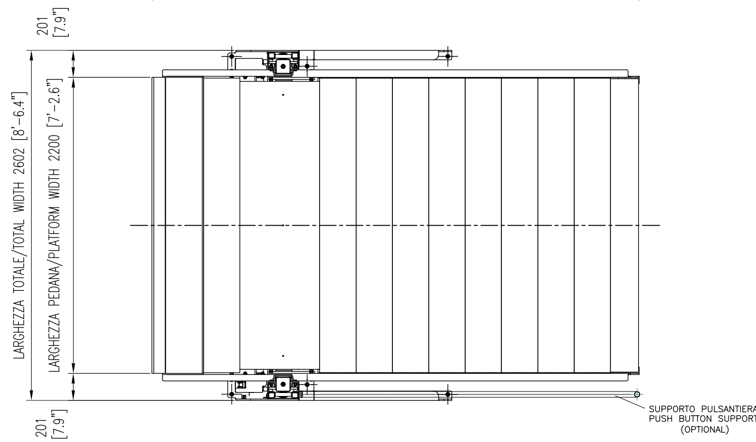
BIPARK 26 H=2050 (80.7") - PLATFORM WIDTH=2200 (86.6")
